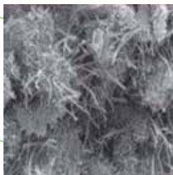
Typische cementbinding (beton C30/37 – schaal 23µm)
